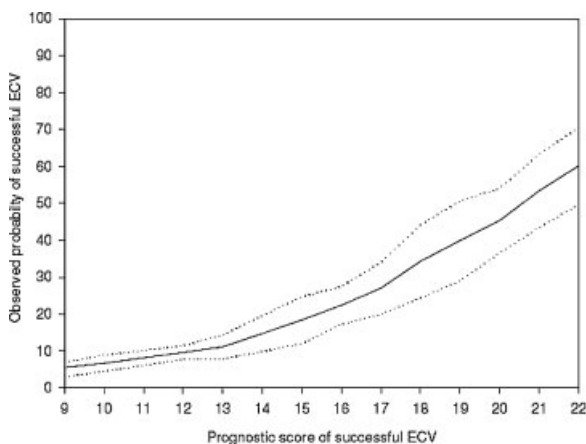
Figure 3 Prognostic score versus chance of successful ECV (95% confidence interval). ECV, external cephalic version.
