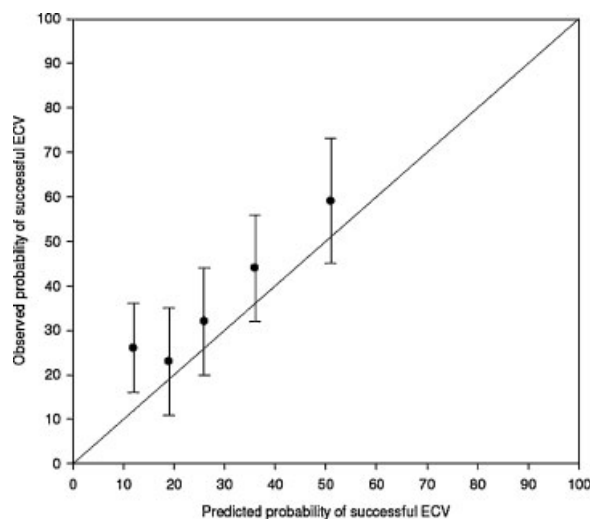
Figure 2 Calibration plot demonstrating the association between the chance of a successful external cephalic version (ECV) as predicted by the logistic model and the observed chance of a successful ECV.
